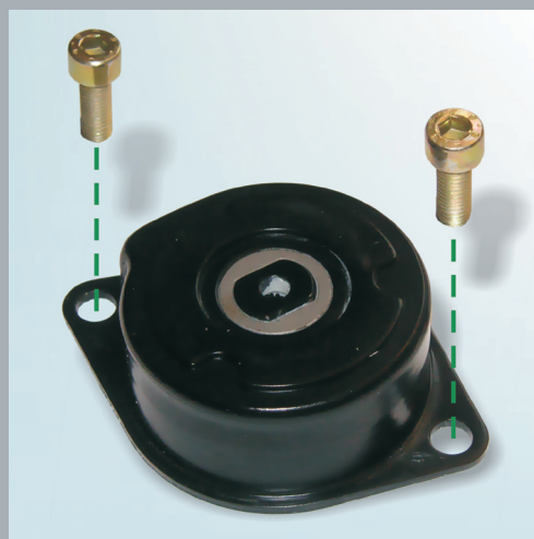
Image 2: Design with two M8x22 bolts
