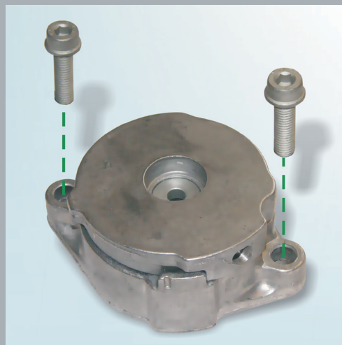
Image 1: Design with two M8x35 bolts
