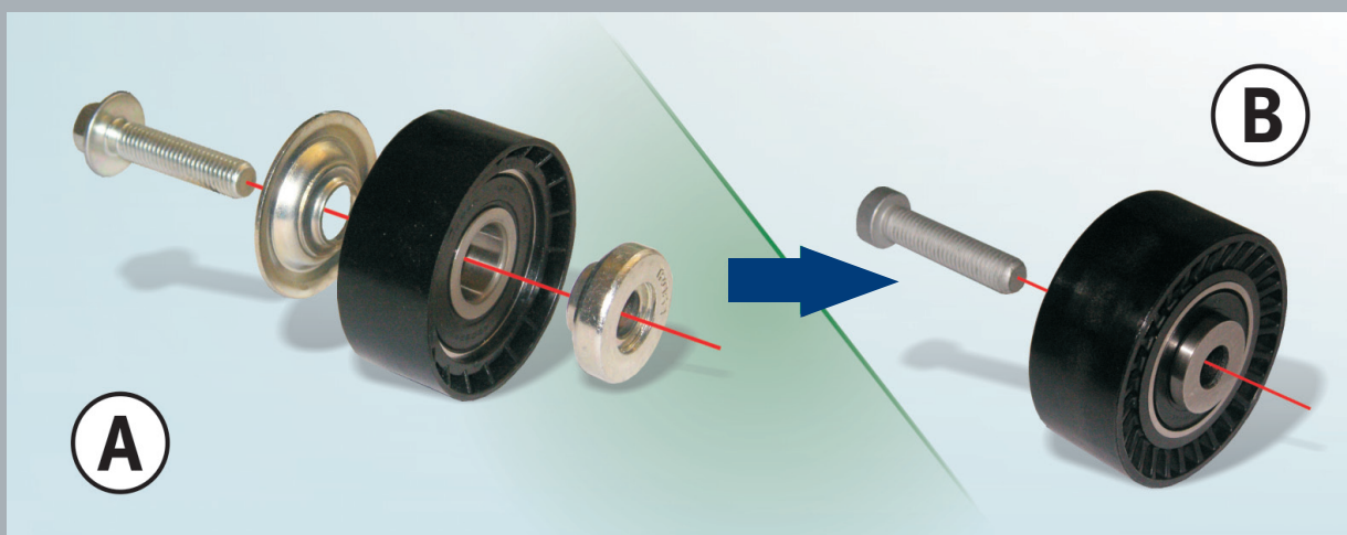
Deflection pulley 55941, previous design (A) and new design (B)
